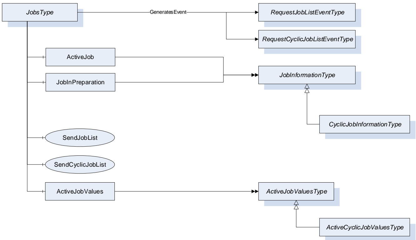
Figure 10 – JobsType Overview
