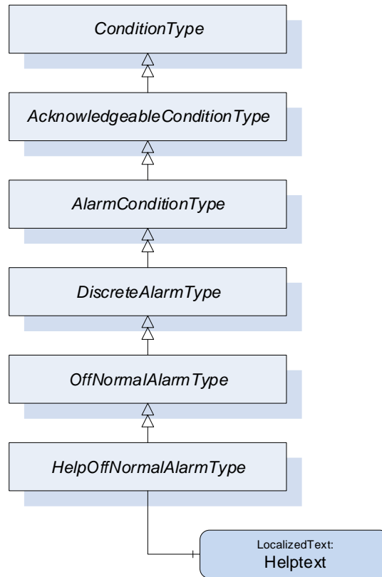
Figure 14 – HelpOffNormalAlarmType Overview
