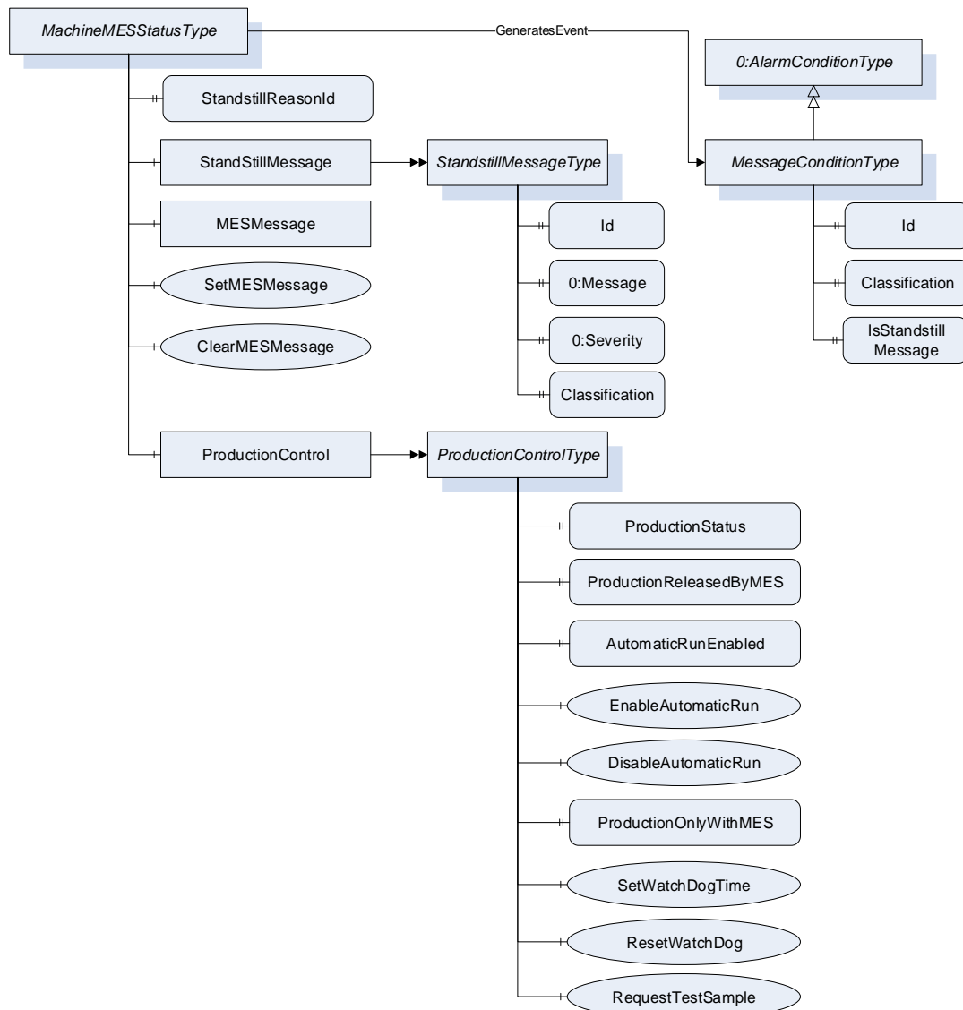
Figure 5 – MachineMESStatusType Overview
