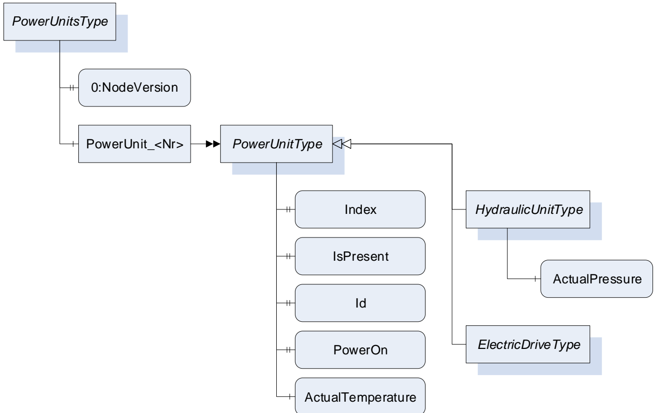
Figure 7 – PowerUnitType Overview
