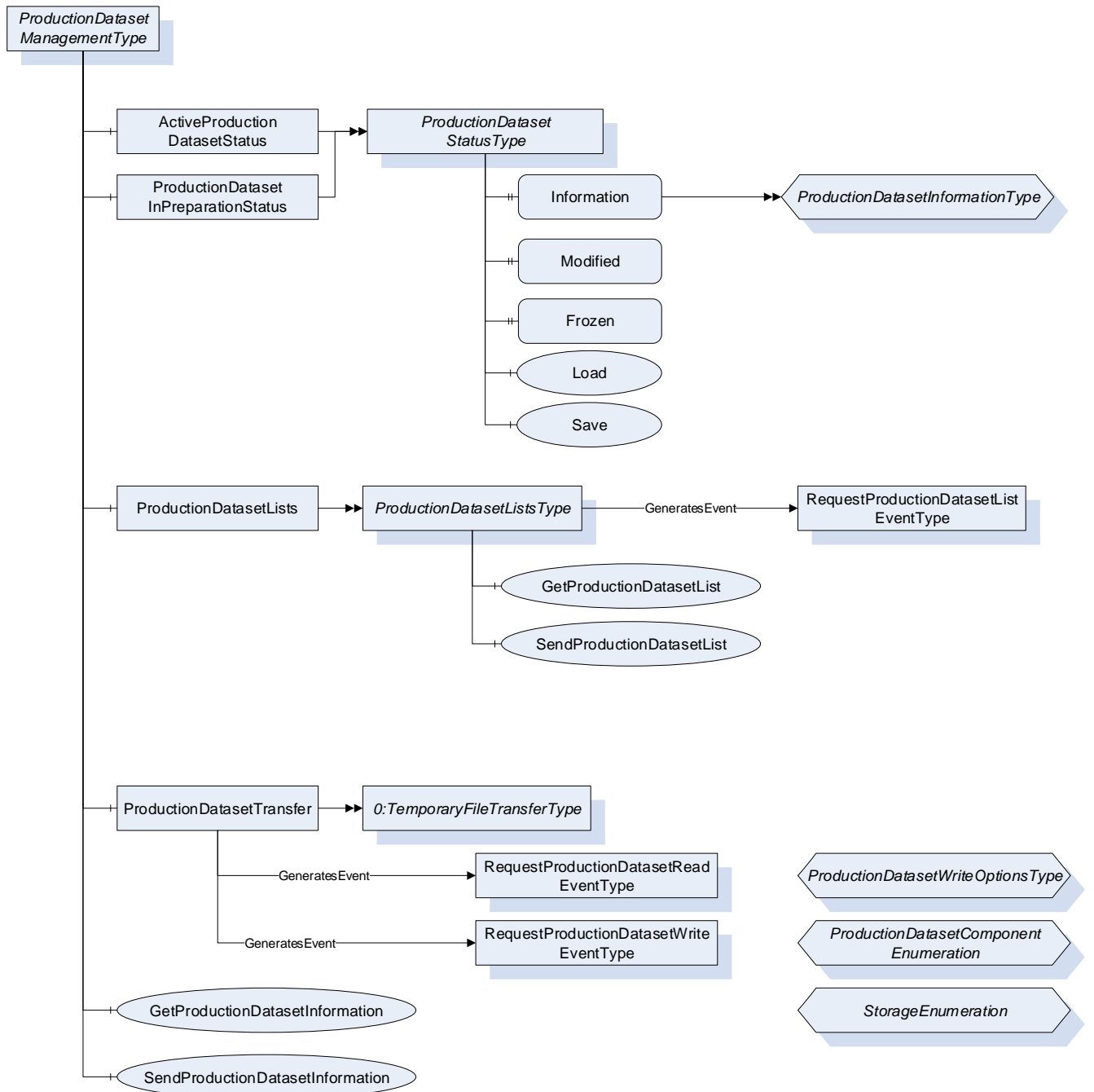
Figure 11 – ProductionDatasetManagementType Overview
