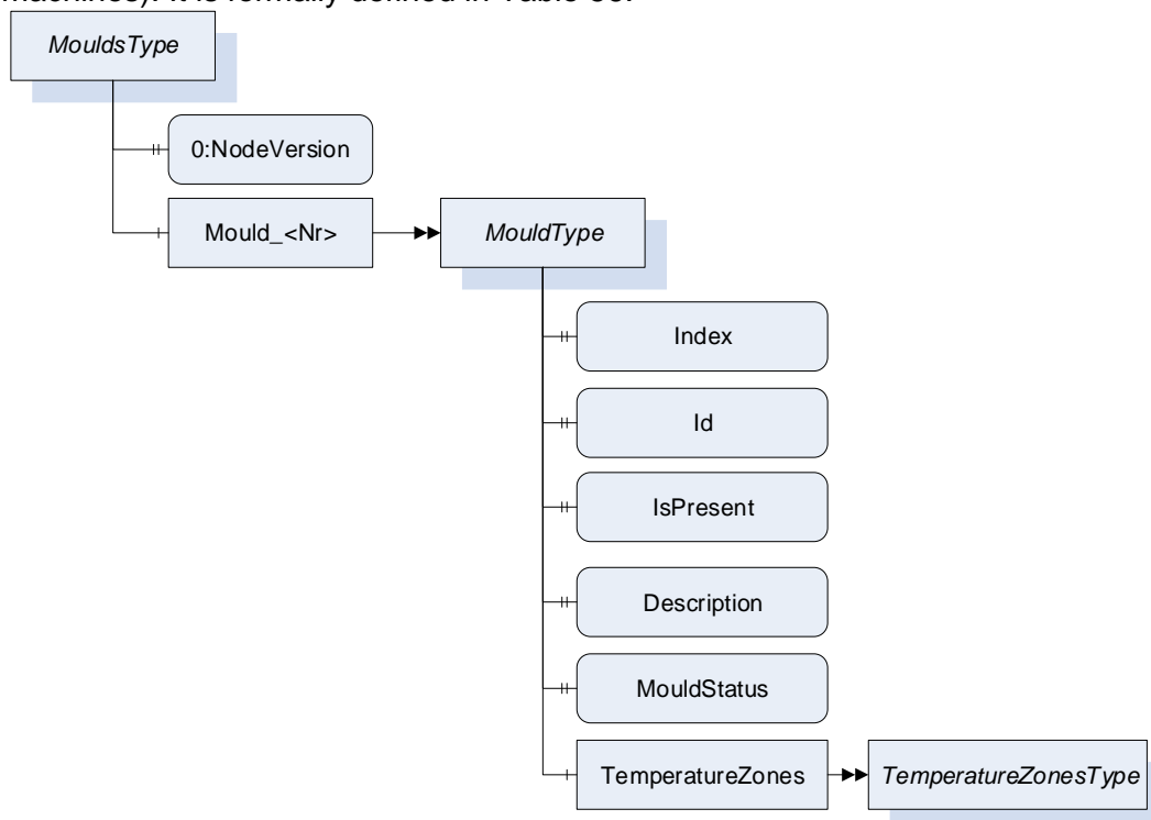
Figure 6 – MouldType Overview
