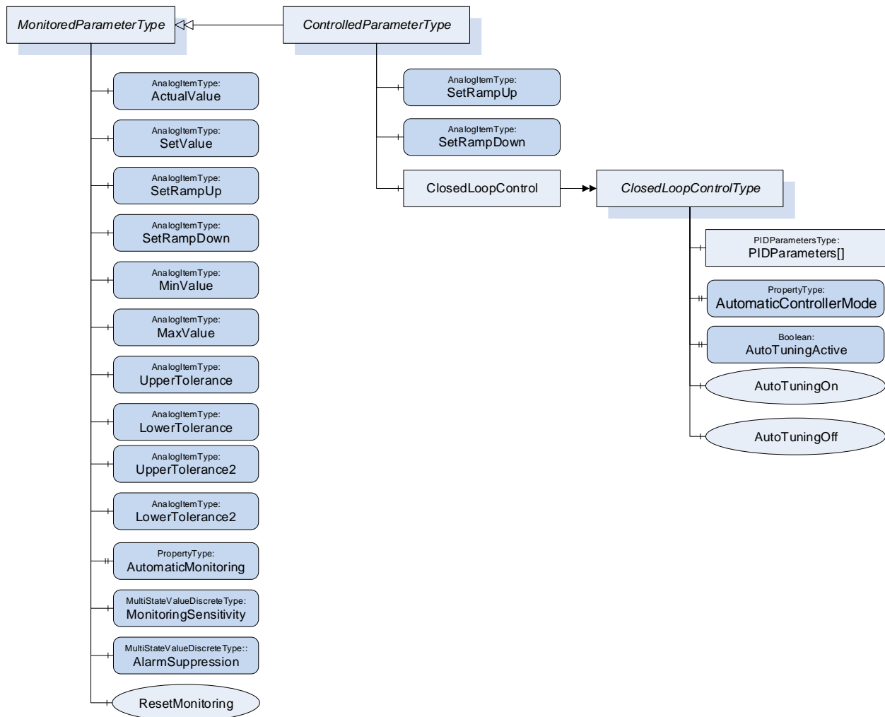
Figure 12 – MonitoredParameterType Overview
