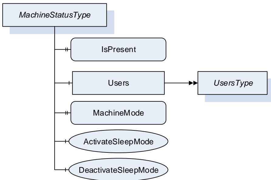
Figure 4 – MachineStatusType Overview
